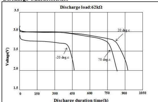
Discharge Characteristics
