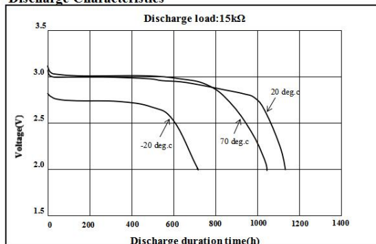
Discharge Characteristics
