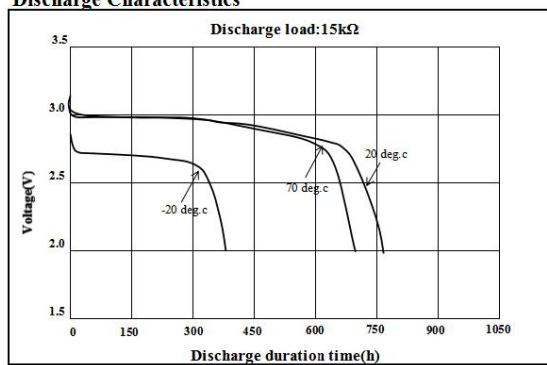
Discharge Characteristics
