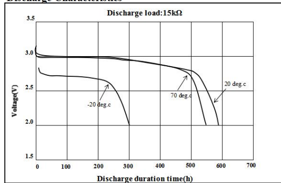
Discharge Characteristics
